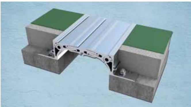
Heavy Duty Flush Mounted Profile
